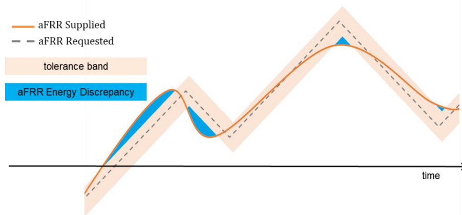
Figure 99 - aFRR Energy Discrepancy
