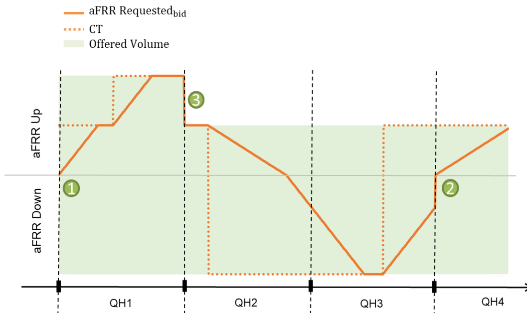
Figure 7 - Determination7 - Determination of aFRR Requested bid
