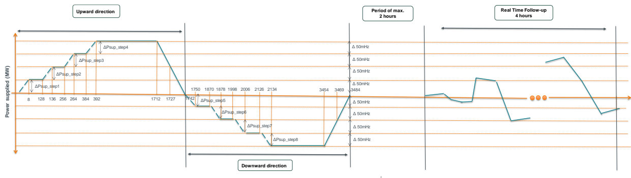
Figure 1: Power profile of the prequalification test
