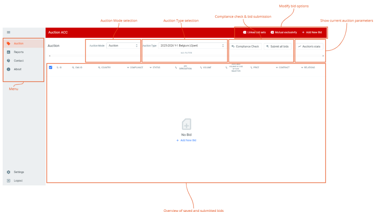
Figure 5: General overview of the CRM Auction interface
