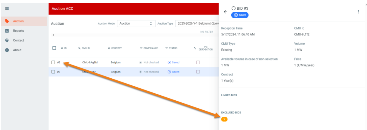
Figure 18: The bid detail menu shows the bid ID(s) of the bid(s) that are mutually exclusive with the selected bid
