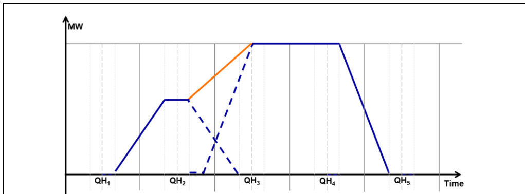
Figure 11: Example of consecutive activation of mFRR Energy Bids part of a same bid group
