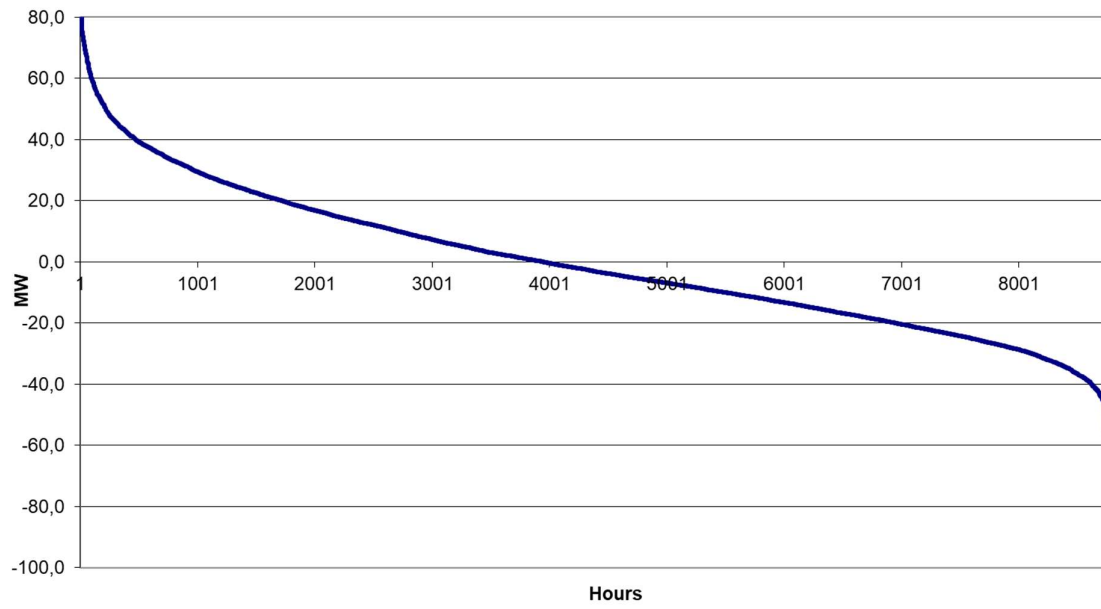
Monotone curve for compensation deficit 2022
