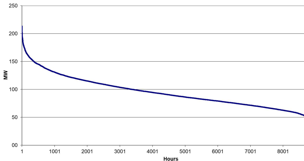
Monotone curve of losses 2022 380-220-150 kV network
