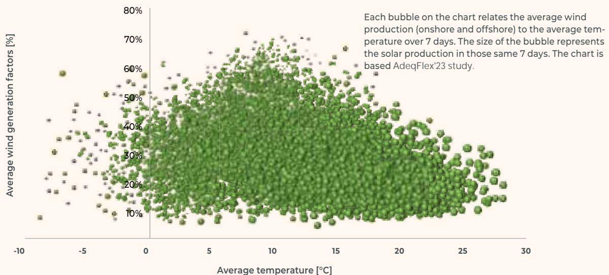
FIGURE J-7 — CORRELATION BETWEEN WIND PRODUCTION, SOLAR PRODUCTION AND TEMPERATURE (7-DAY AVERAGE)
