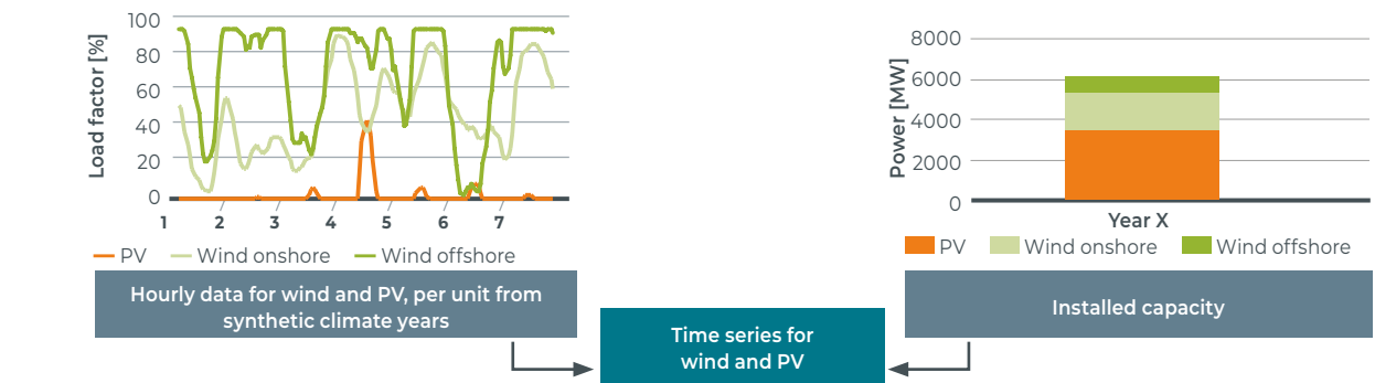
FIGURE J-6 — GENERATION TIME SERIES FOR WIND AND PV. STARTING FROM HOURLY PRODUCTION FOR EACH CLIMATE YEAR, THESE CAN BE SCALED UP WITH A GIVEN INSTALLED CAPACITY TO CREATE THE PRODUCTION TIME SERIES
