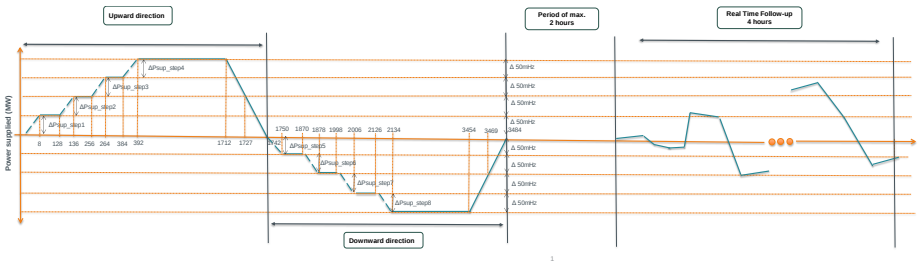
Figure 1: Power profile of the prequalification test
