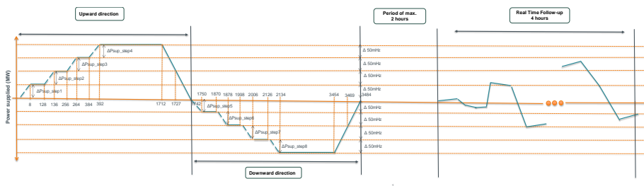
Figure 1: Power profile of the prequalification test
