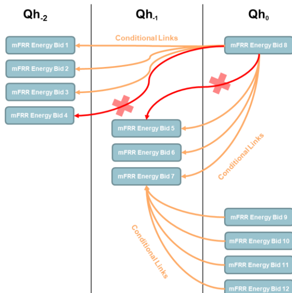
Figure 5: Illustration of allowed and not-allowed conditional links
