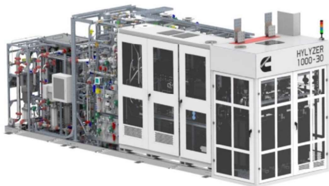
Figure 2: 5MW PEM electrolyser, product Hylyzer 1000
