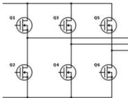
Figure 5: Three-phase full bridge active rectifier topology
