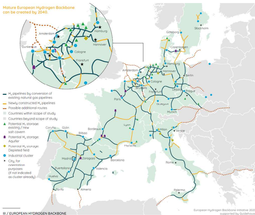
Figure 18: Proposed EU hydrogen backbone from reference 31
