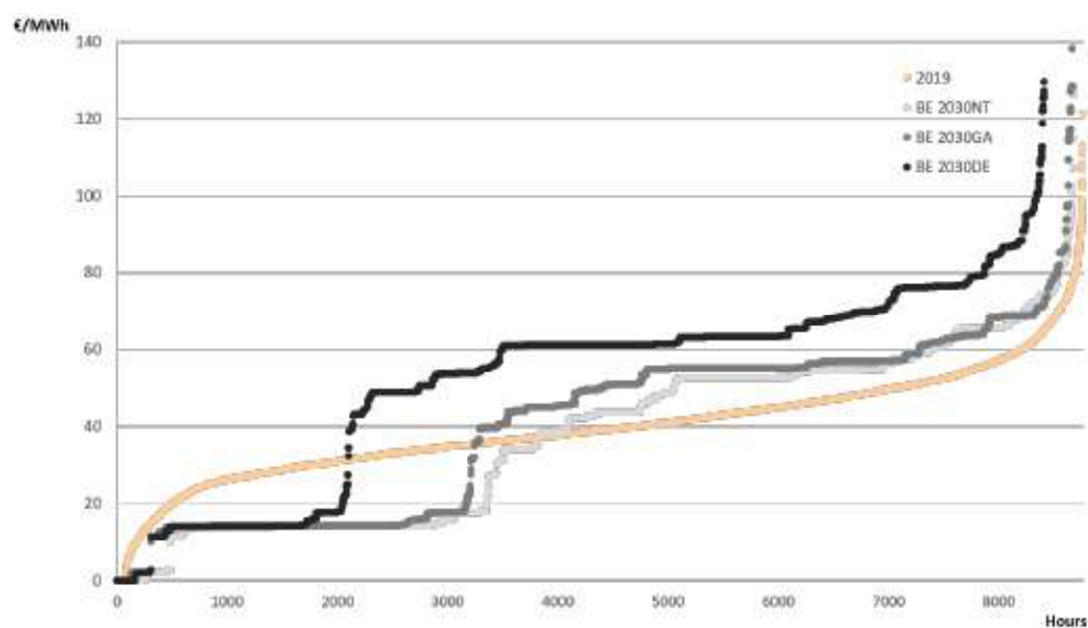
Figure 11: Modelled 2030 electricity prices for Belgium.
