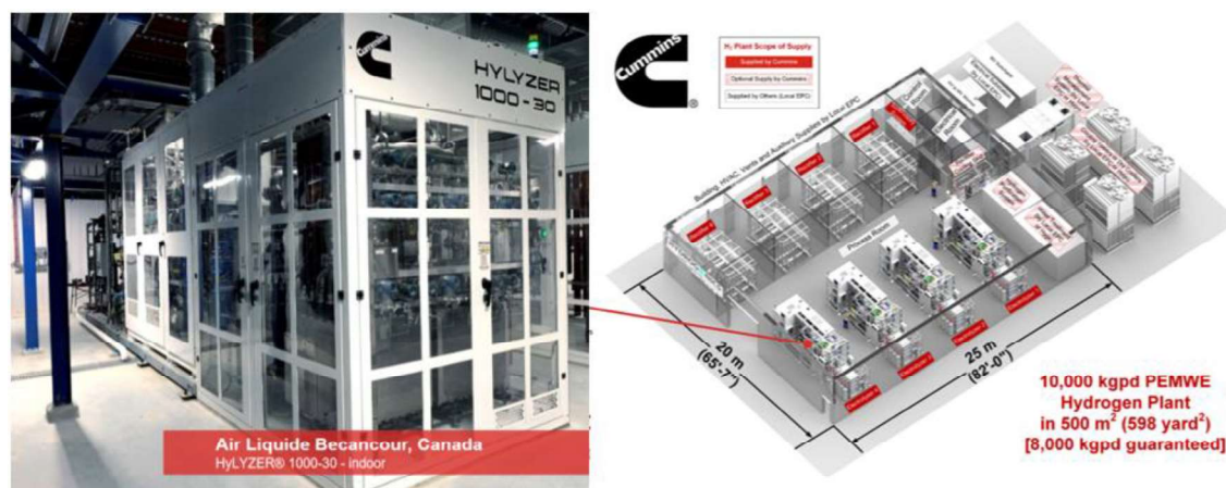
Figure 3: 20MW electrolyser plant, based on the Hylyzer 1000 product
