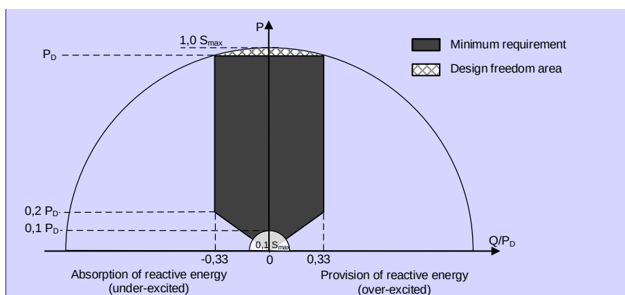
Capability curve for SPGM type B
