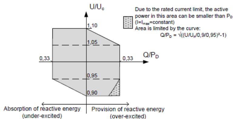
Figure 4: U-Q/P D profile for type B SPM in order to visualize reactive power requirements for voltages different from 1pu.
